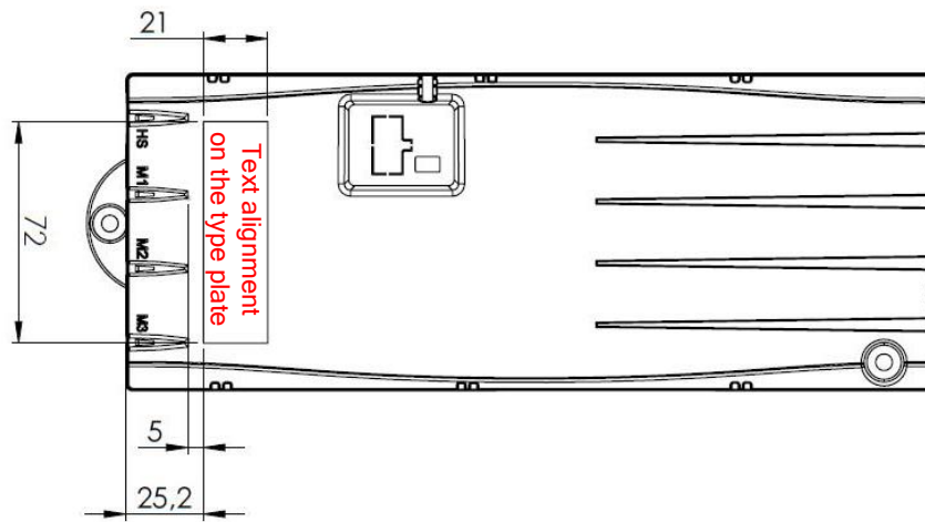
Figure 7: Text alignment on the type plate of COMPACT eco -DIN
